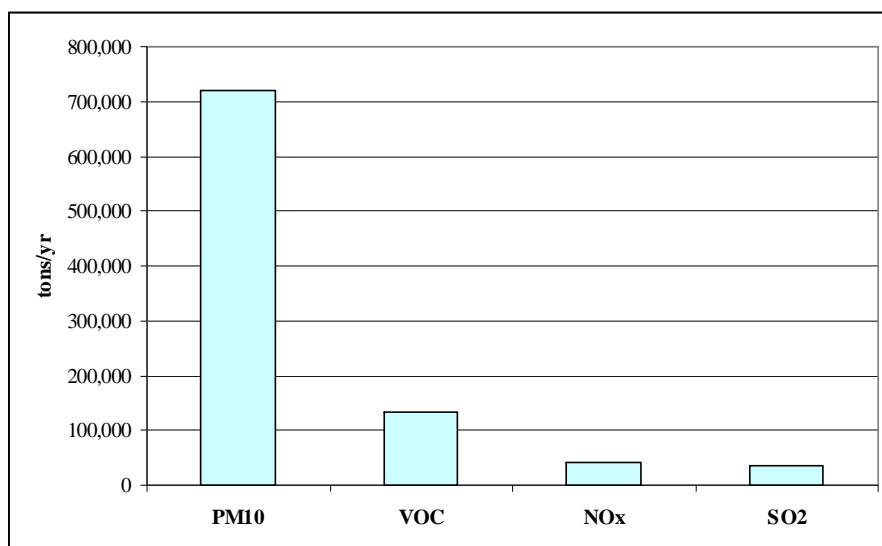
Figure 7.1 2002 Emissions of Pollutants Contributing to Regional Haze from Kansas Nonpoint Sources
