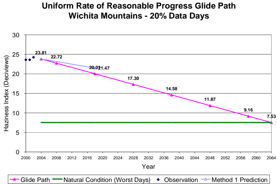
Figure 8.3 URP Glide Path for Wichita Mountains Class I Area with 2018 Projected Results – 20% Worst Days
